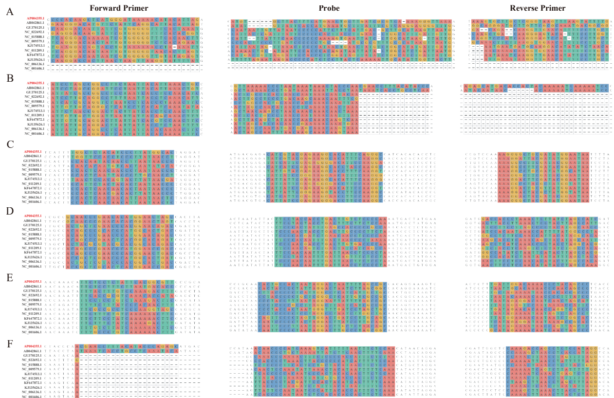
Figure 1. Sequence variation alignments of the RPA and qPCR primer/probe set in mitochondrion genome of the Atractosteus spatula and the 11 comparative species. A. RPA1; B. RPA2; C. qPCR1; D. qPCR2; E. qPCR3; F. qPCR4. The correspondence between sequences and names is as follows, AP004355.1: A. spatula ; AB042861.1: Lepisosteus oculatus ; GU370125.1: Nile tilapia ; NC_022692.1: Rhinogobius giurinus ; NC_015888.1: Tachysurus fulvidraco ; NC_009579.1: Coilia nasus ; KJ174513.1: Acipenser sinensis ; NC_011209.1: Misgurnus anguillicaudatus ; KF647872.1: Hemibarbus maculatus ; KJ135626.1: Pseudorasbora parva ; NC_006136.1: Carassius auratus ; NC_001606.1: Cyprinus carpio .
