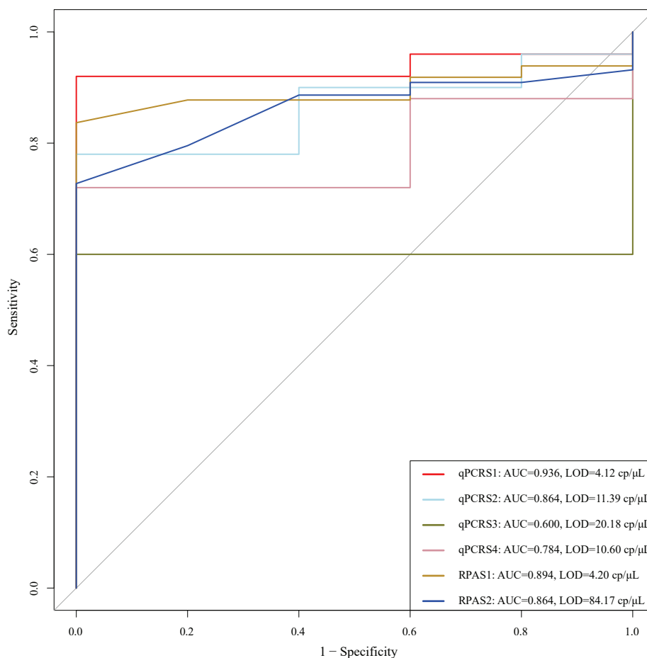
Figure 7. Receiver operating characteristic (ROC) curve of RPA and qPCR detection assays. AUC represents the area under the ROC curve, the AUC range from 0.5 to 1, when AUC is more than 0.9 indicated a relatively high accuracy, with AUC more than 0.7 refers the detection method performs well. LOD refers to the minimum concentration of the target analyte that can be detected from the sample by a specific analytical method at a confidence level of 95%.
