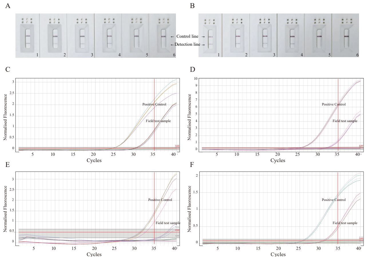
Figure 8. On field test of RPA and qPCR assay. RPAS1 (A) and RPAS2 (B): Lane1: positive control; Lanes2-4: three technical replicates of A. spatula field water eDNA; Lane 5: eDNA from semi-closed lake as negative control; Lane 6: blank control. For qPCR detection assay, except qPCRS3 (E), qPCRS1 (C), qPCRS2 (D) and qPCRS4 (F) achieved a 100% detection rate with all four technical replicates being detected.
