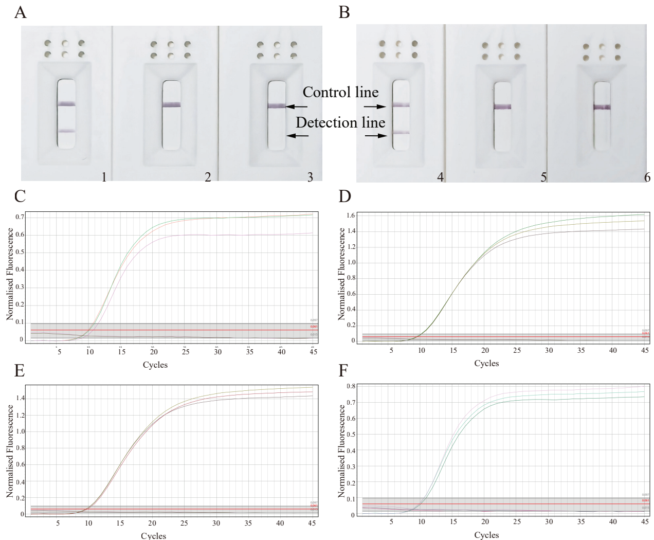
Figure 3. Assessment of the specificity of probes. RPAS1 (A) and RPAS2 (B), Lane 1, 4: Genomic DNA of A. spatula ; Lanes 2, 5: mixed DNA from 11 non-target fish species; Lanes 3, 6: blank controls. Only genomic DNA being detected within qPCR1 (C), qPCR2 (D), qPCR3 (E), qPCR4 (F).
