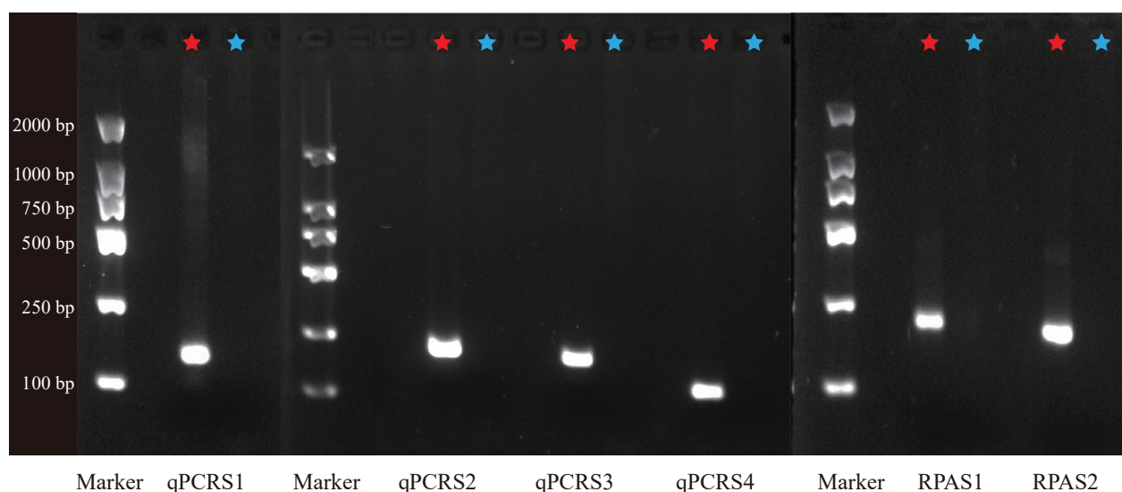
Figure 2. Gel electrophoresis pattern of primer specificity. The red star represents amplification of A. spatula genomic DNA, and the blue star represents amplification of DNA mixture from 11 background fishes.
