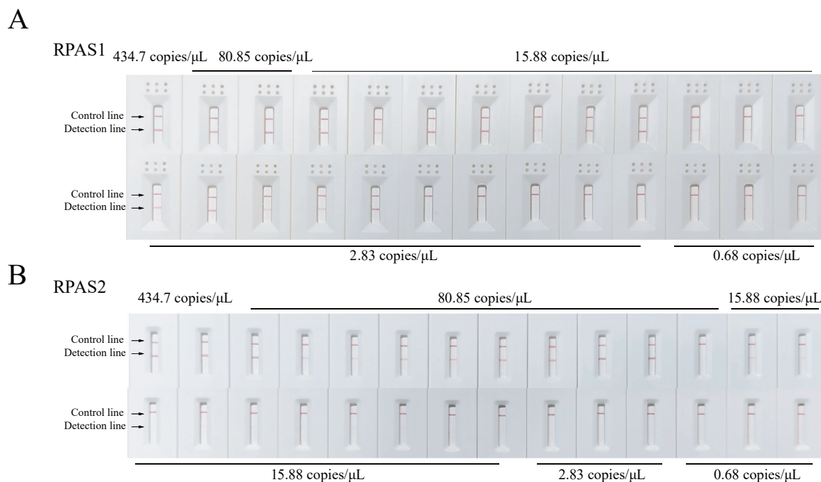
Figure 6. Assessment of the sensitivity of primer-probe pairs of RPA-LFD. A. For RPAS1; B. For RPAS2. Each sample was detected with ten technical replicates at different concentration.
