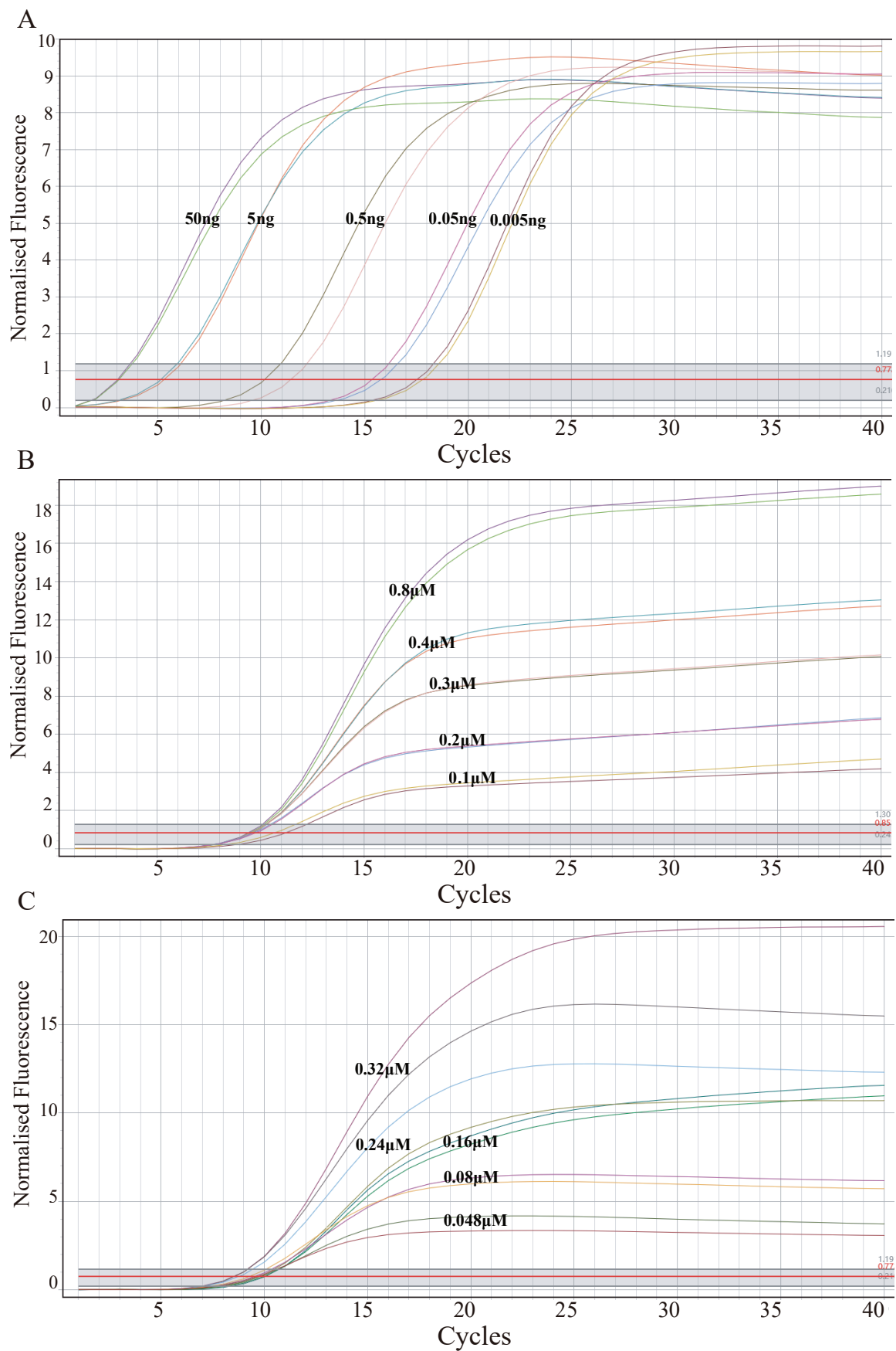
Figure 5. Examination of appropriate concentration in internal quality control system for qPCR. A. Amount of DNA template added in qPCR mixture; Concentration of primer ( B ) and probe ( C ) added in qPCR mixture.
