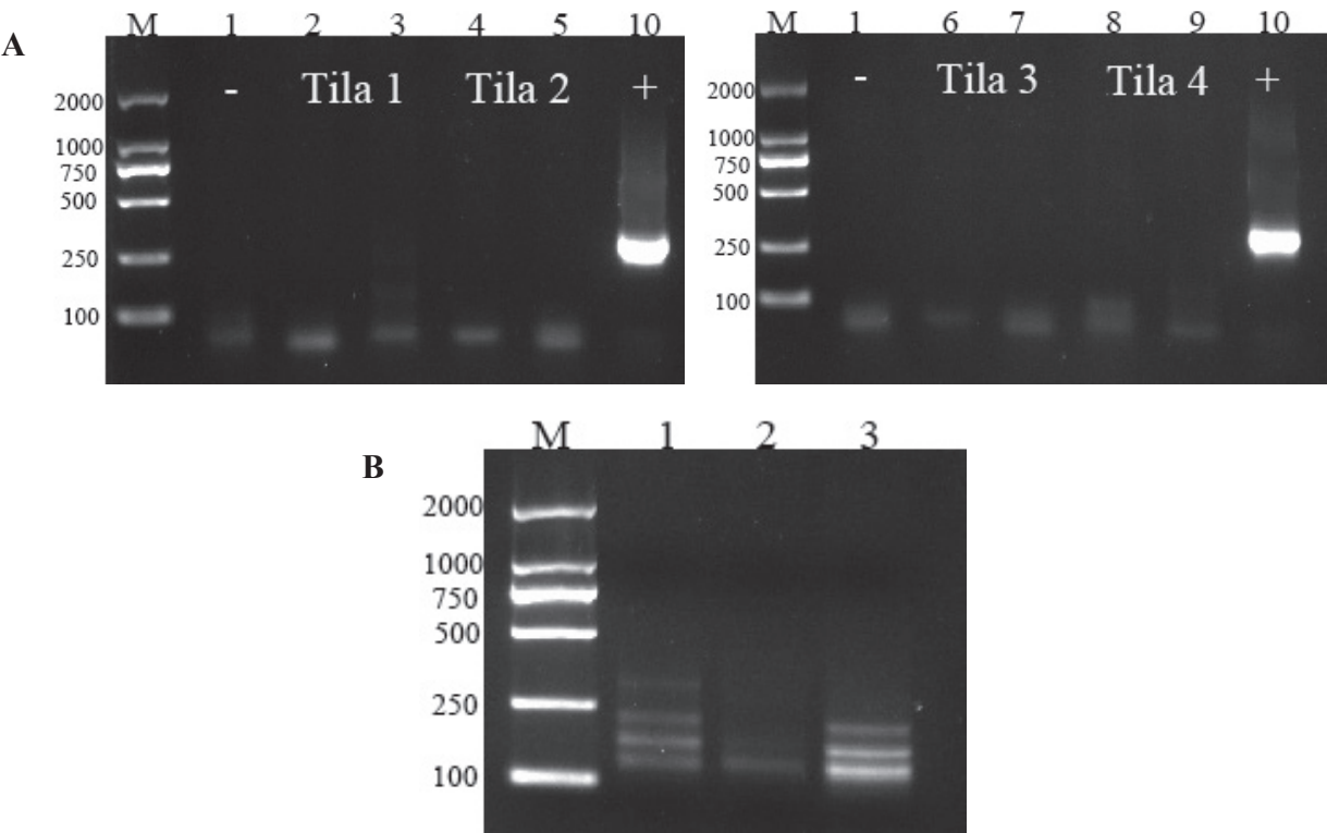
Figure 3. A. Specificity testing of the four tilapia-specific primers. M: marker; lane 1 is a blank control (primer: Tila 1), lanes 2–3 are Tila 1, lanes 4–5 are Tila 2, lanes 6–7 are Tila 3, lanes 8–9 are Tila 4, and lane 10 is a positive control using O. niloticus DNA (primer: tele02); paired lanes show the results of the 20 species mixture and Cichlasoma managuense . B. Multiplex PCR amplification using the mixed primer set (Tila1–Tila4). M: marker; lane 1: O. niloticus tissue DNA; lane 2: sample collected from natural water; lane 3: water sample collected from an aquaculture tank containing tilapia.
