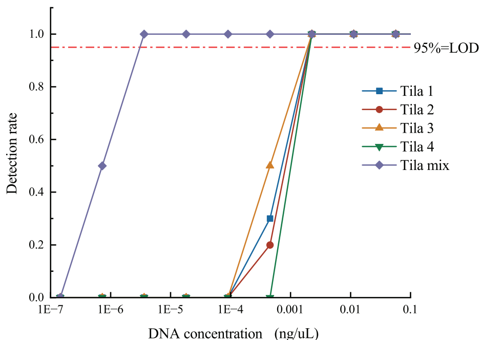
Figure 4. Detection rates of individual primer sets (Tila1, Tila2, Tila3, and Tila4) and the primer combination (Tila-mix) at different DNA concentrations (ng/μL). This figure illustrates the 95% limit of detection (LOD) and the consistency of detection at low template concentrations. Tila-mix refers to the combination of all four primer pairs.
